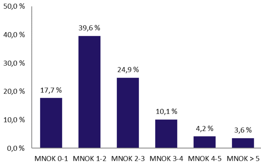
Pool notional
